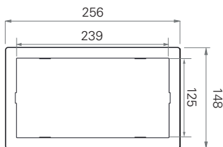
Dimensions in mm (Recessed kit for ceiling)
